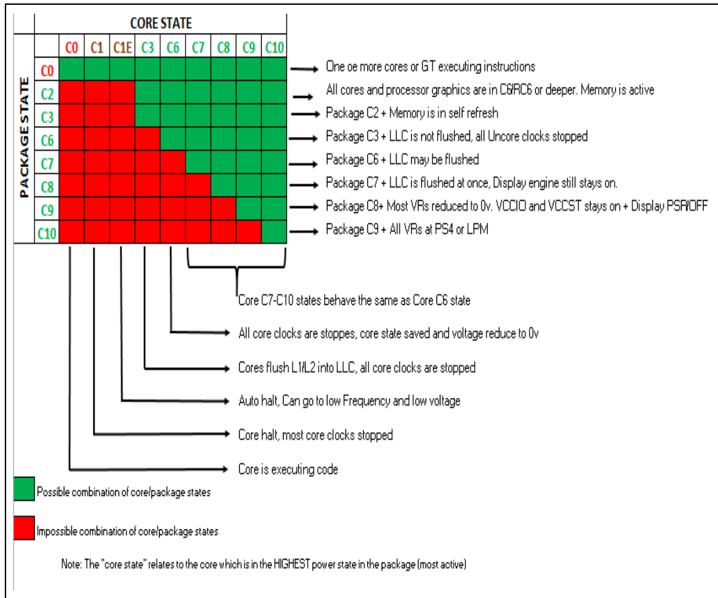
Figure 4-2. Processor Package and IA Core C-States
