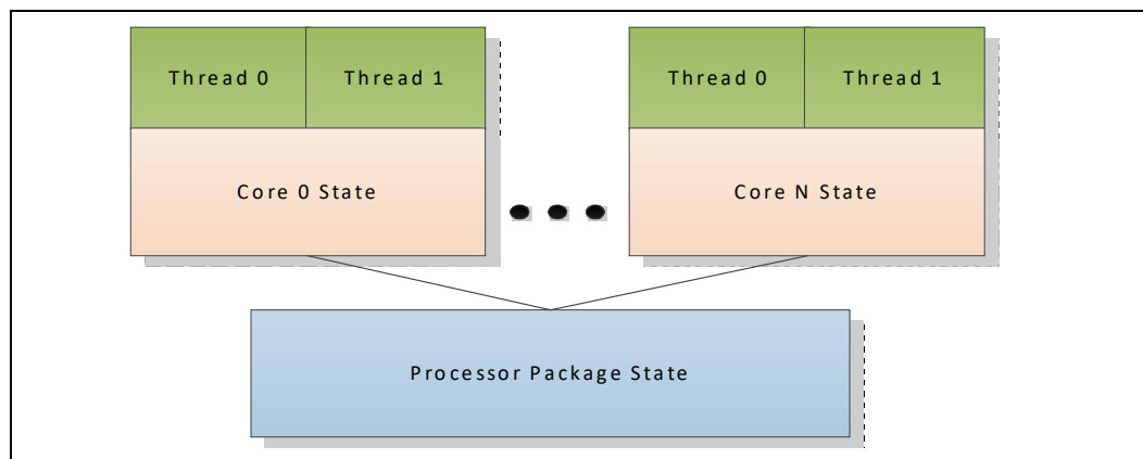
Figure 4-3. Idle Power Management Breakdown of the Processor IA Cores
