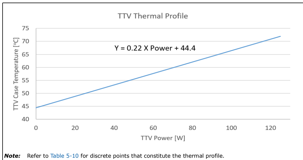
Figure 5-2. Thermal Test Vehicle Thermal Profile for PCG 2015D Processor
