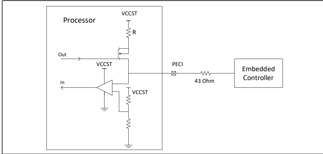
Figure 2-9. Example for PECE EC Connection
