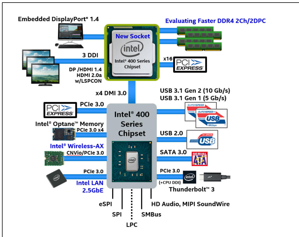
Figure 1-1. H/S-Processor Line Platforms
