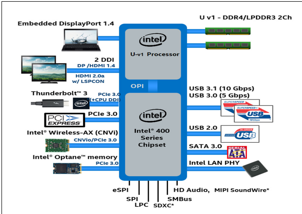
Figure 1-2. U-Processor Line Platform
