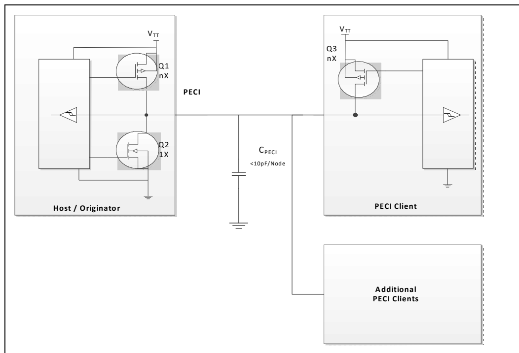
Figure 2-8. Example for PECE Host-Clients Connection
