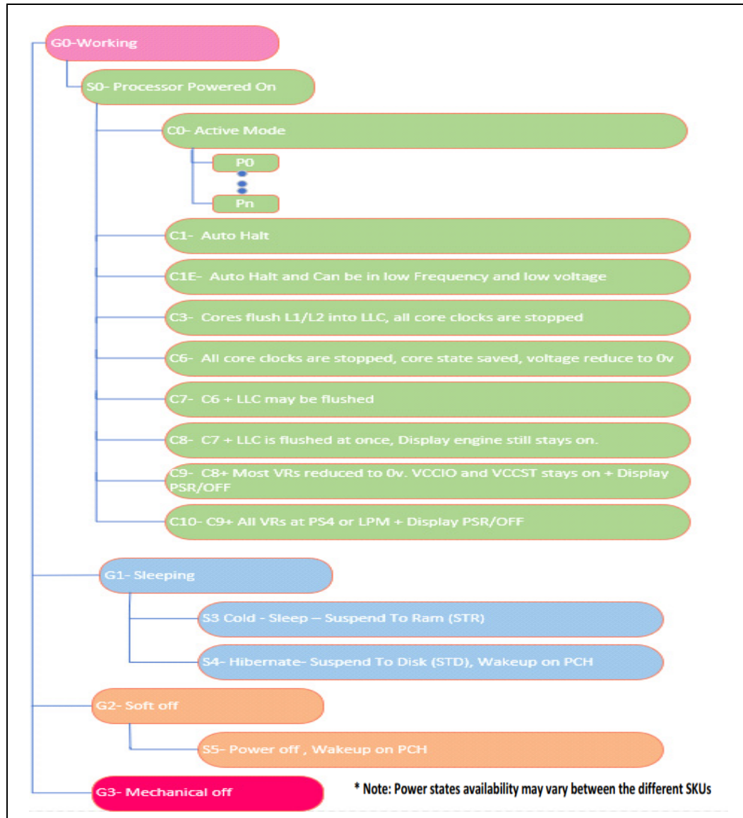
Figure 4-1. Processor Power States
