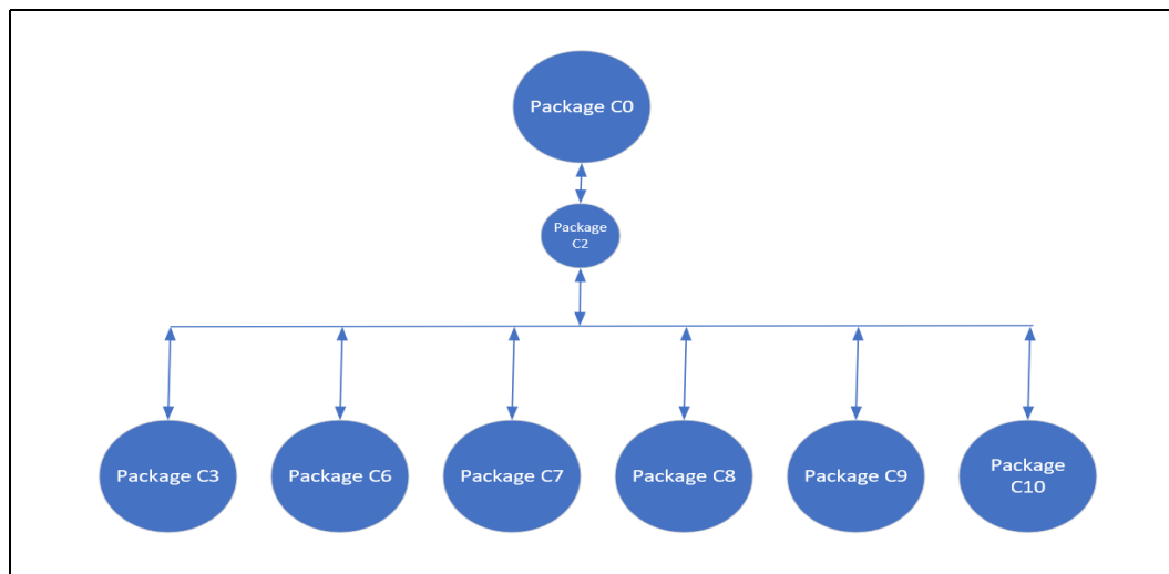
Figure 4-4. Package C-State Entry and Exit
