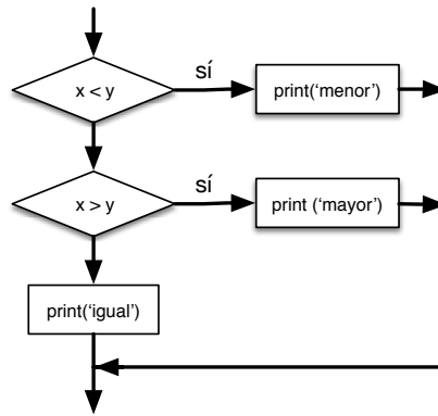
Figure 3.3: If-Then-Elsef Logic
